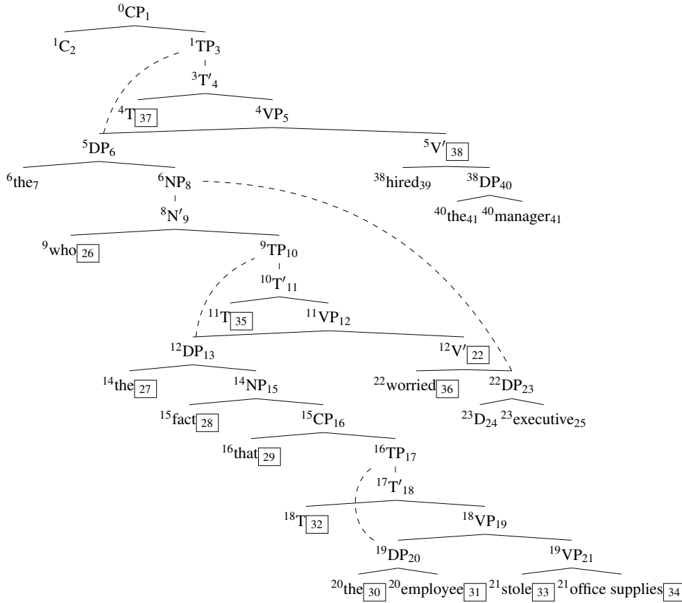
Figure 3: Relative clause containing a sentential complement; Max = 33/33, MaxLex = 33/17, Box = 14/11, BoxLex = 12/9
